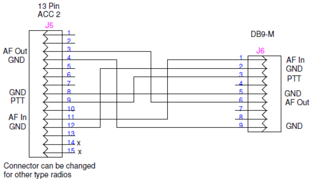
Figure 6.99 TS-2000 ACC-2 to DB9 Adapter
