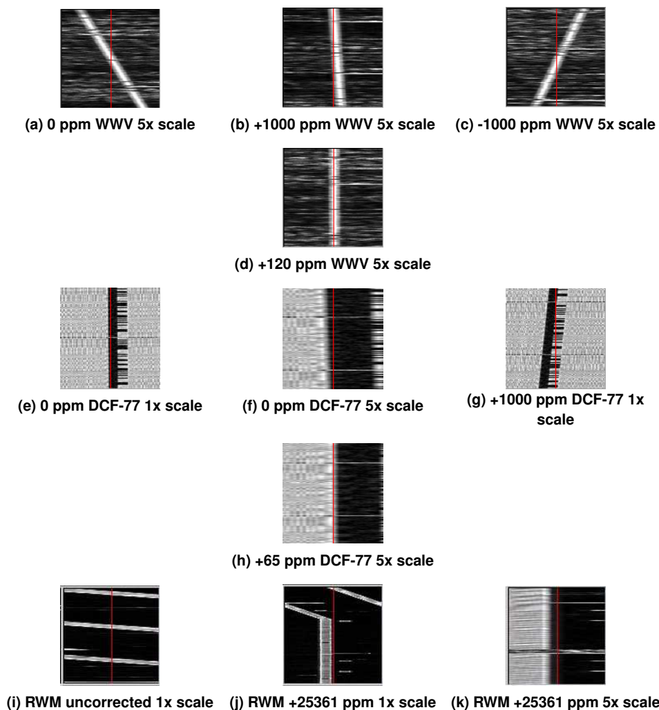
Figure 6.12 PSK Digiscopes
