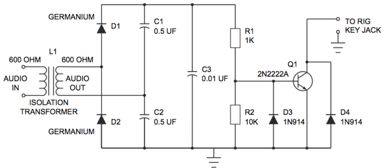
Figure 6.2 CW Keying Circuit
