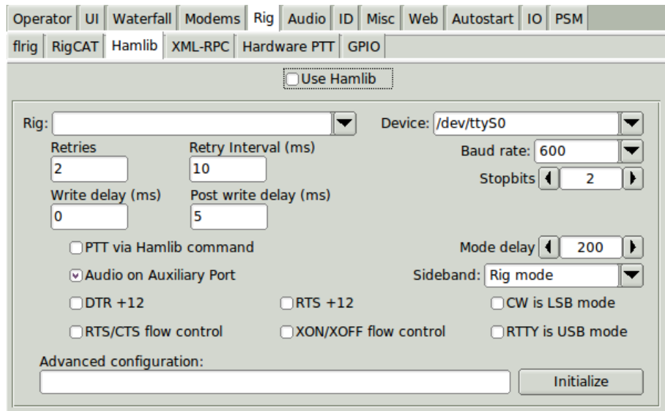
Figure 2.10: Hamlib CAT Control
