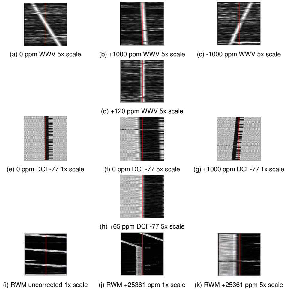
Figure 6.13: PSK Digiscopes
