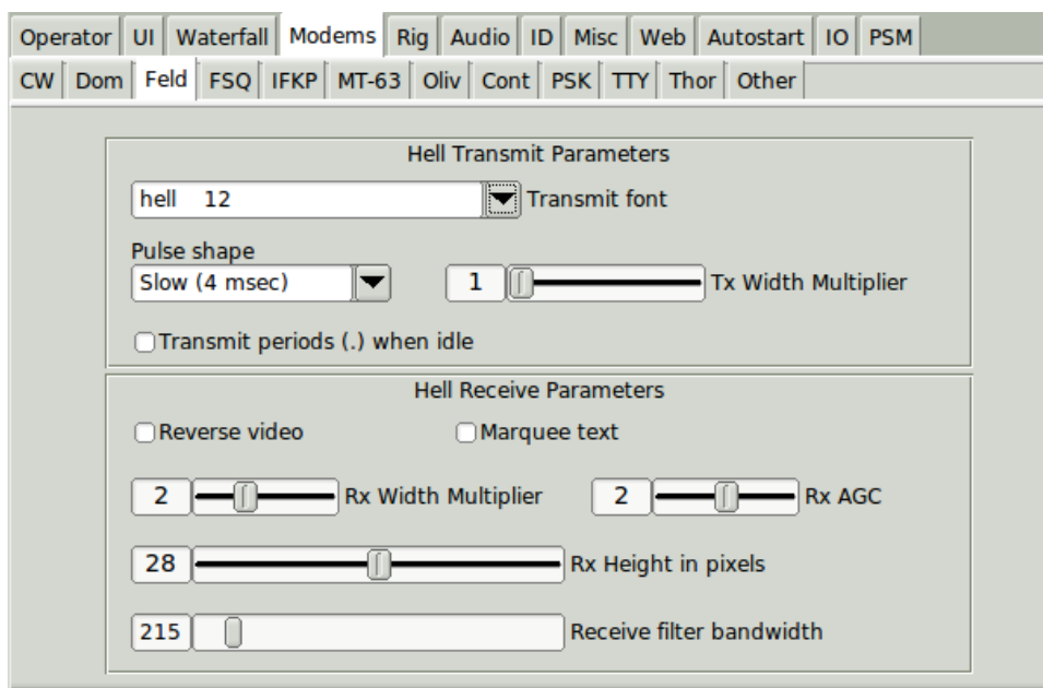
Figure 2.119: Feld Hell Config Panel
