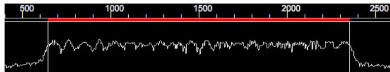
Figure 5.55: PSK63R20C signal transmitting text data - oscilloscope view
