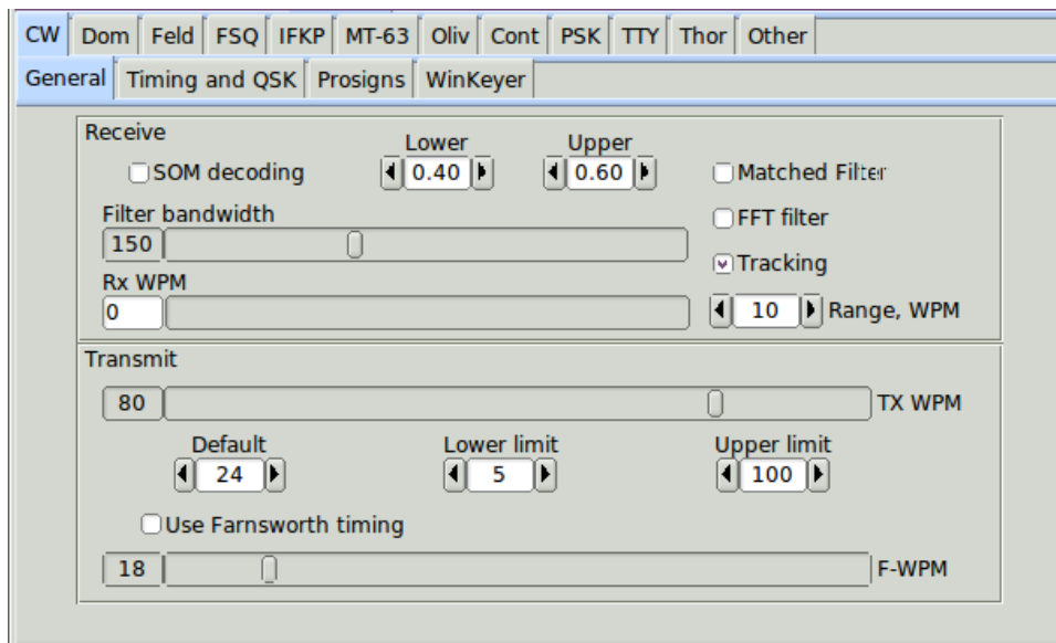
Figure 2.109: General CW Configuration
