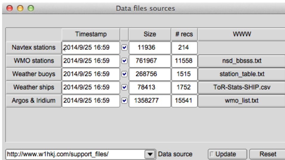
Figure 6.98: Downloading and updating data files used for various decodings
