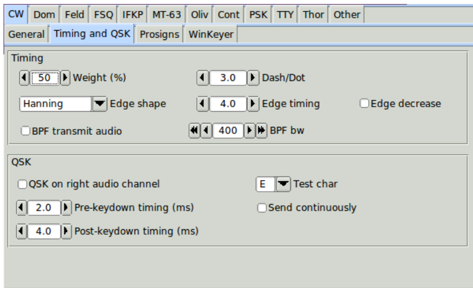
Figure 6.2: Timing and QSK
