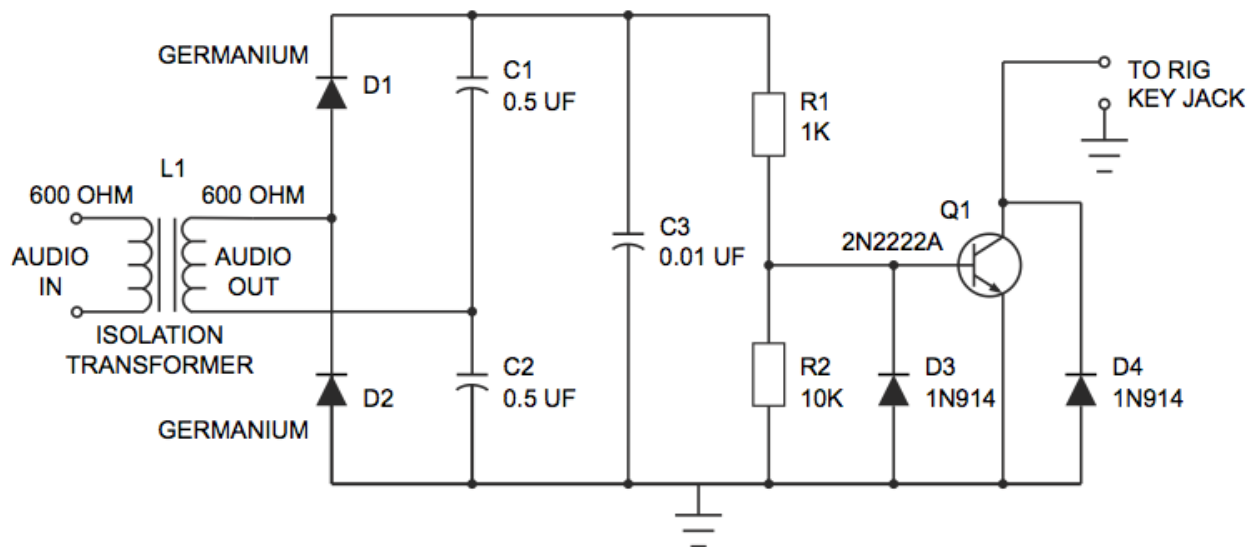
Figure 6.3: CW Keying Circuit
