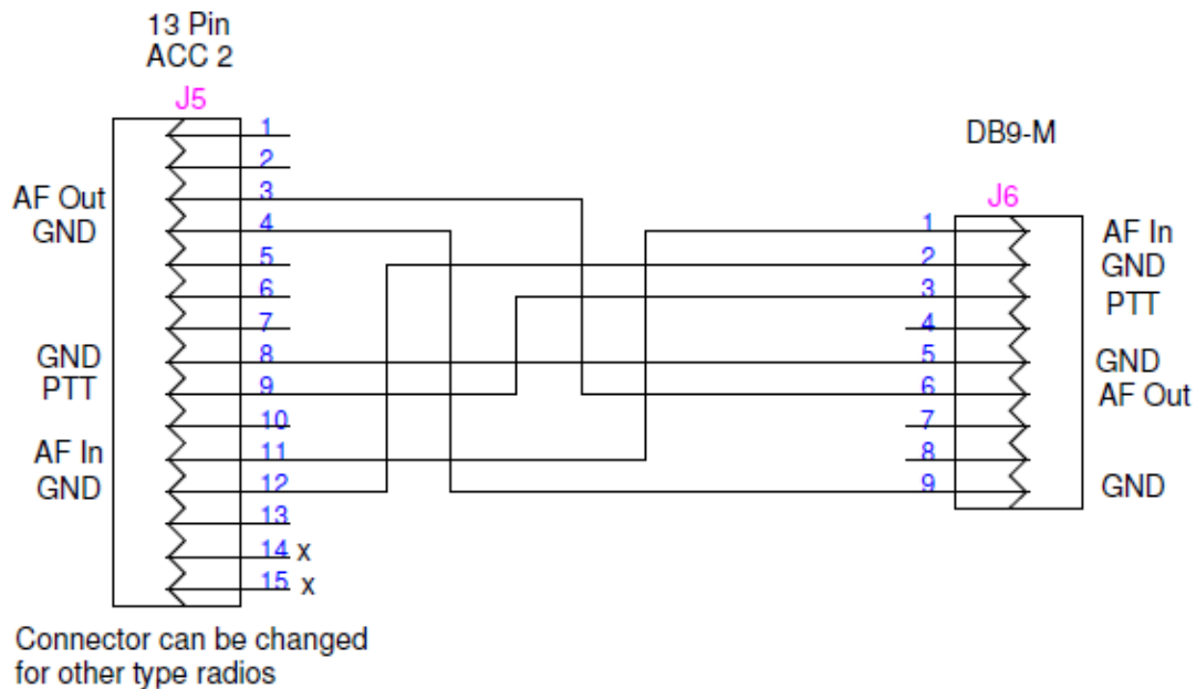
Figure 6.101: TS-2000 ACC-2 to DB9 Adapter
