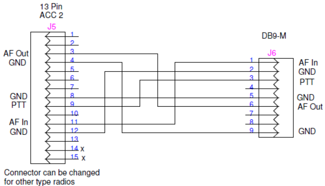
Figure 6.96: TS-2000 ACC-2 to DB9 Adapter
