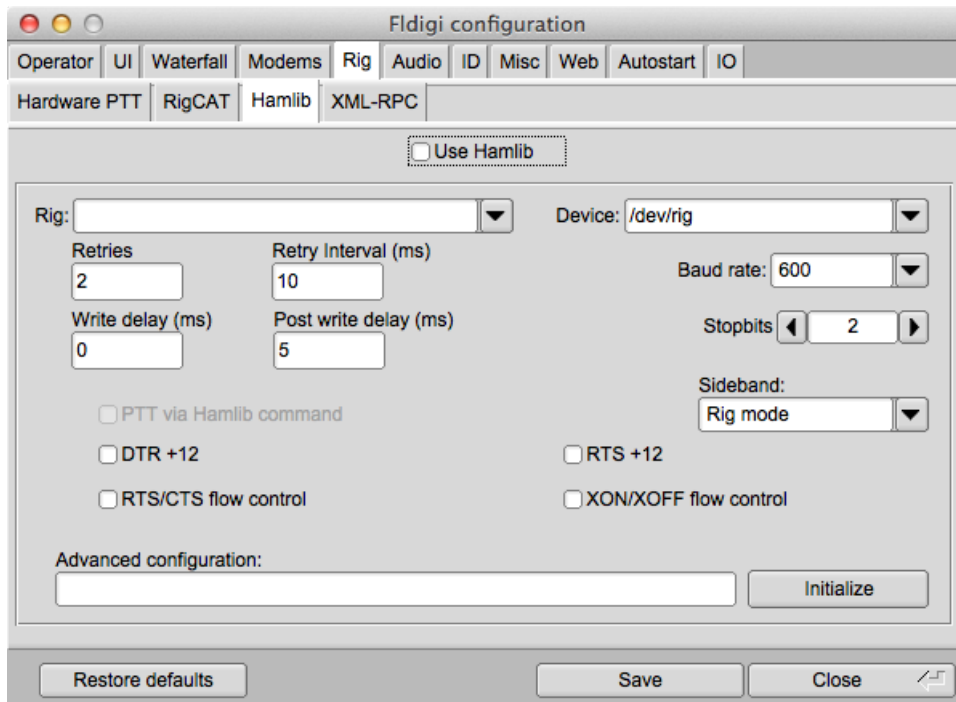
Figure 6.83: Hamlib CAT Control
