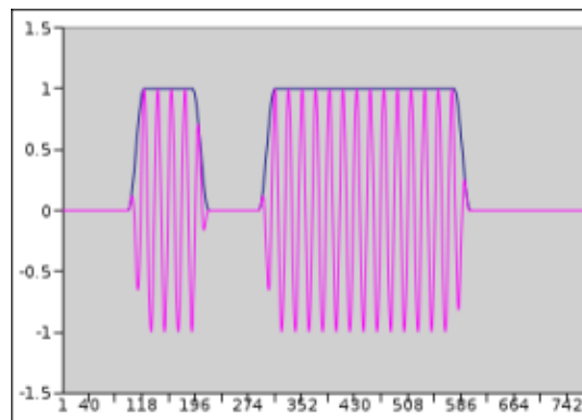
Figure 2.109: Dash/Dot = 3.0, Edge = 3 msec
