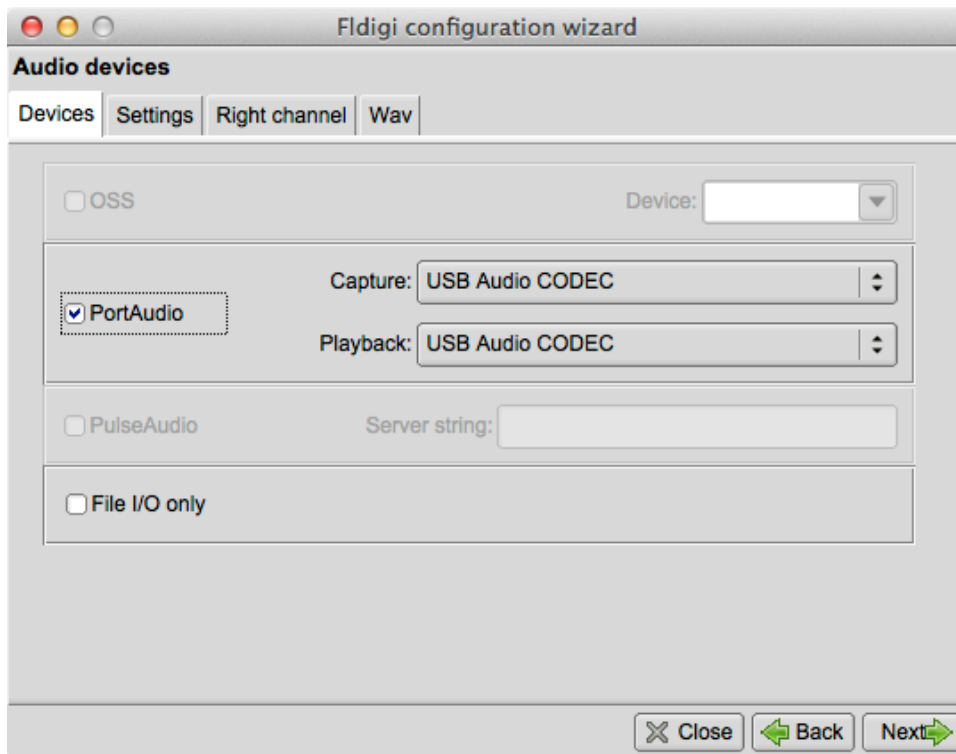
Figure 2.35: Sound Card Configuration
