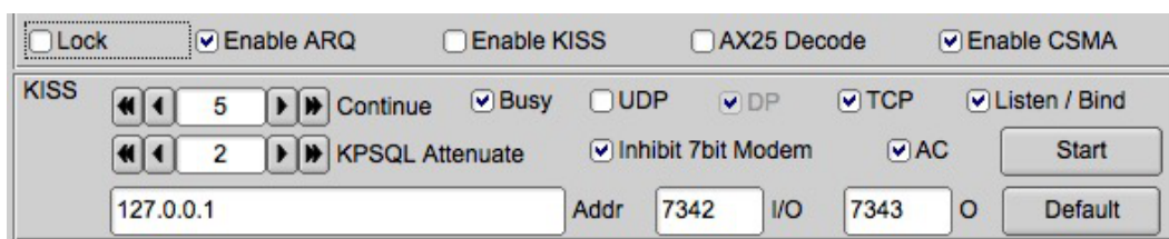
Figure 2.30: KISS IO Panel Options
