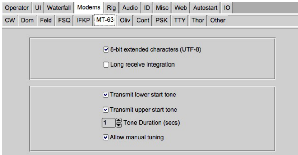
Figure 2.132: Modems MT63 Config Panel
