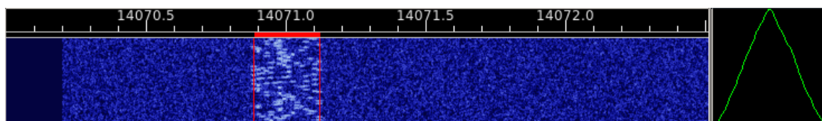
Figure 5.33: MFSK16 signal
