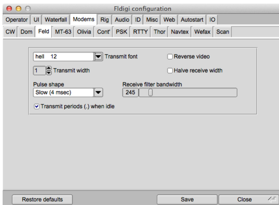
Figure 2.115: Feld Hell Config Panel
