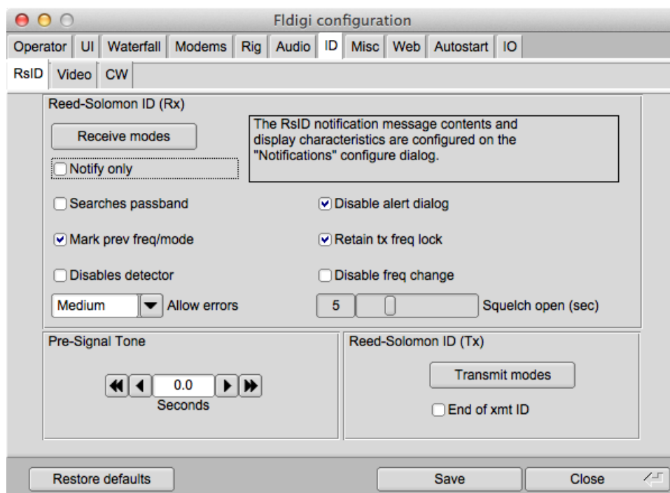
Figure 2.116: RSID Config Panel
