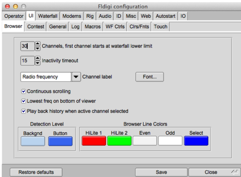
Figure 2.64: UI Browser Configuration
