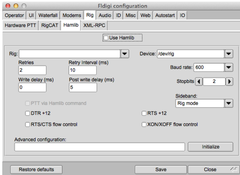
Figure 2.13: Hamlib CAT Control
