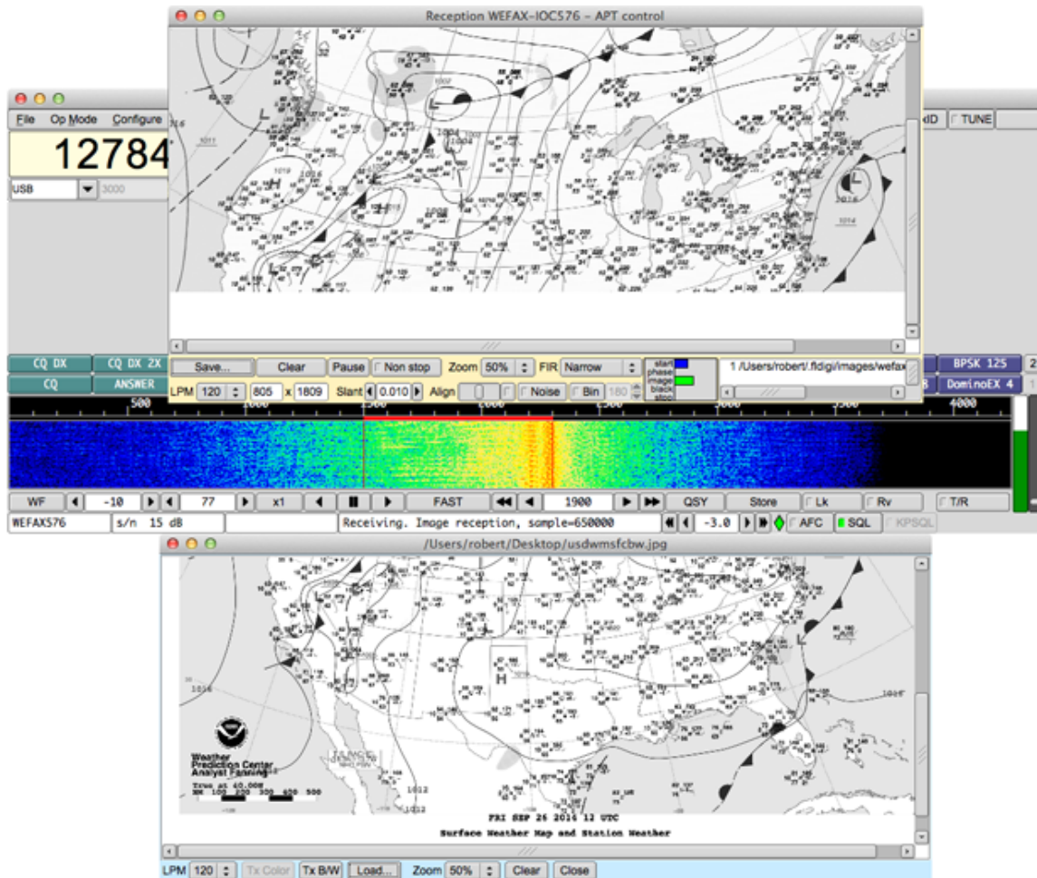
Figure 2.92: Detached WEFAX Window
