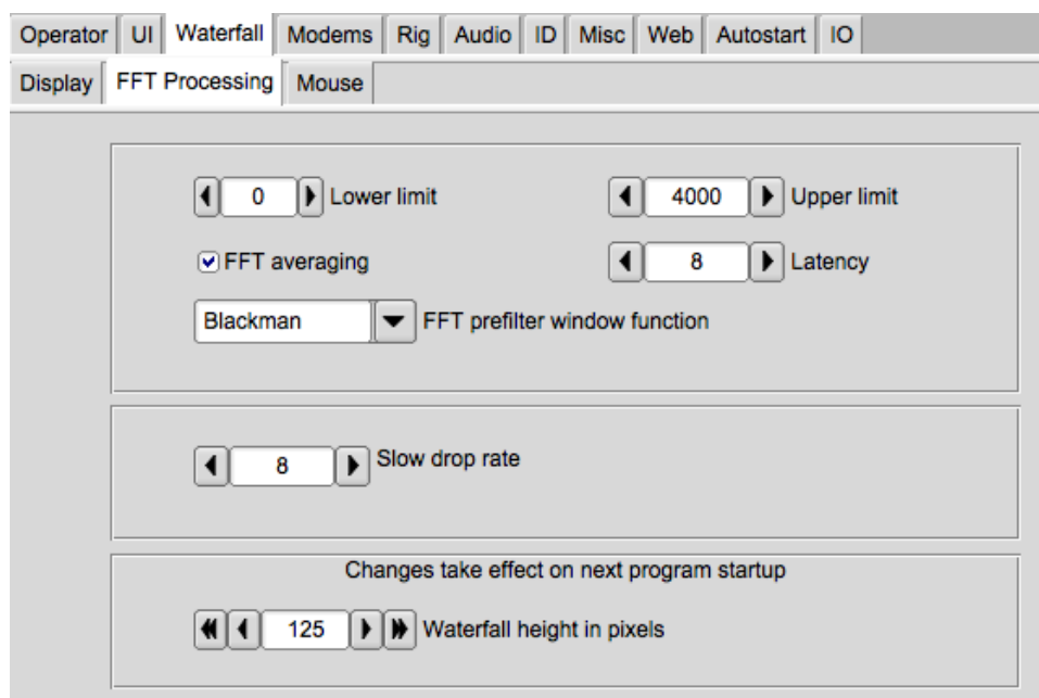
Figure 2.88: UI Waterfall Display
