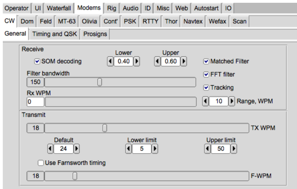
Figure 2.105: General CW Configuration
