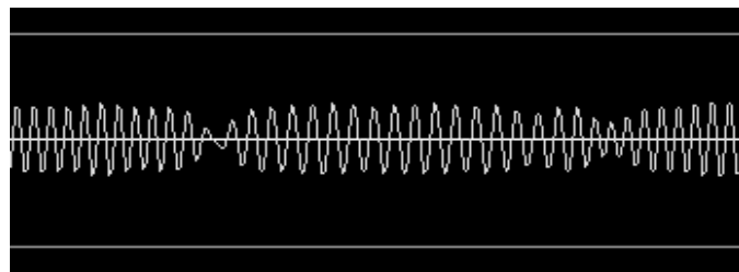
Figure 5.63: AFSK signal
